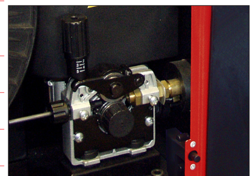
Foto del vano bobina con trainafilo a 2 rulli Photo of the spool compartment with 2-roller wire feeder.
